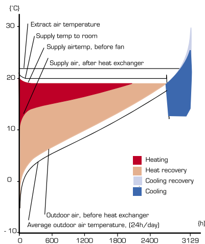
Recuterm® plate exchanger: at 57% efficiency
