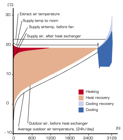
Regoterm® thermal wheel: at 76% efficiency
