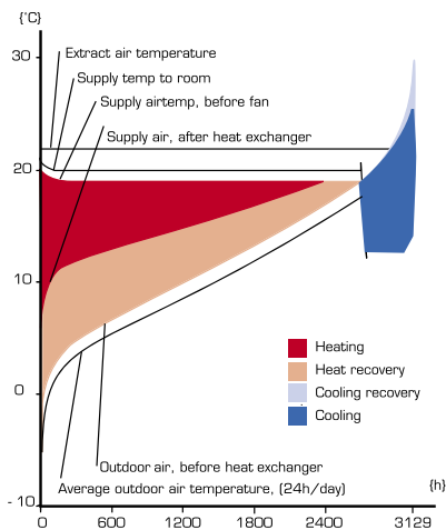
Ecoterm® run-around coil: at 42% efficiency
